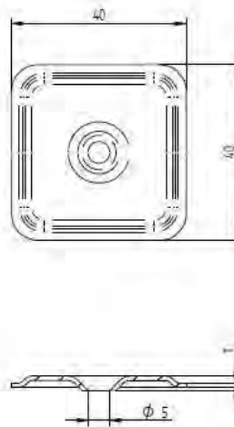
Eurofast DVP-K-4040H
