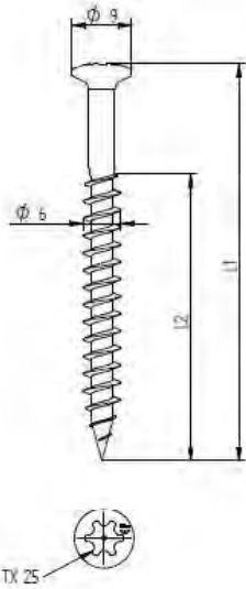
VRF Eurofast GBS 6,0 x L
