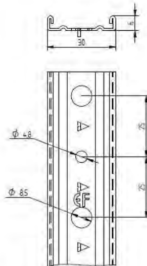
Eurofast EDF-BAR-FB
